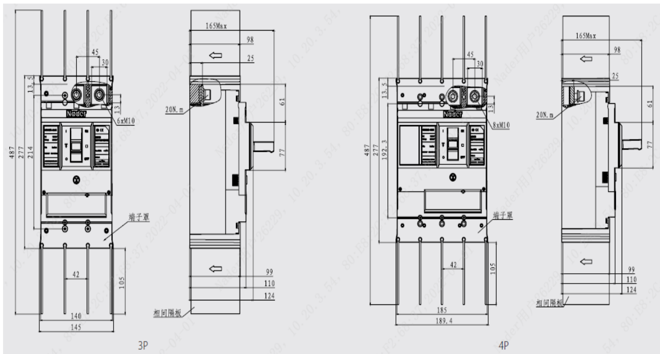
Fig.10 Size of terminal cover
