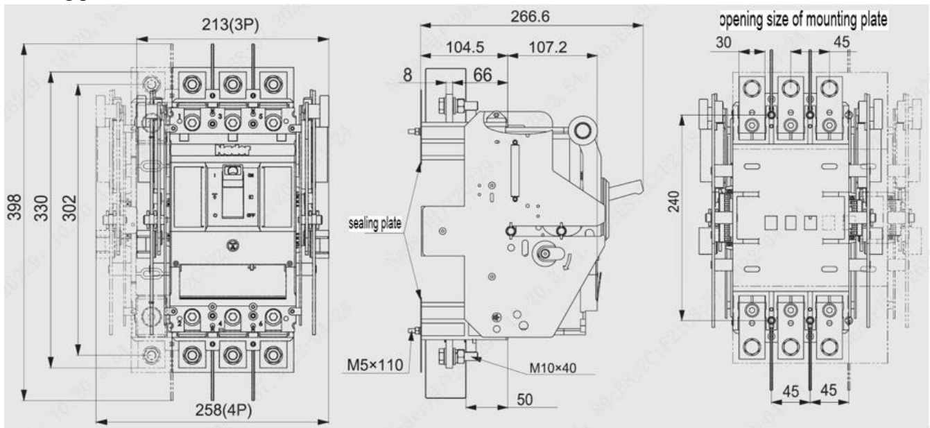
Fig.17 3P、4P Outline dimensions drawing of withdrawable front panel board wiring products
