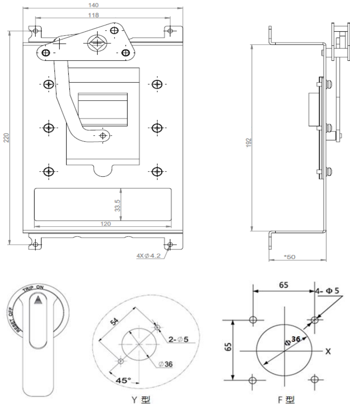
Fig.21 Installation opening diagram of rotary handle
