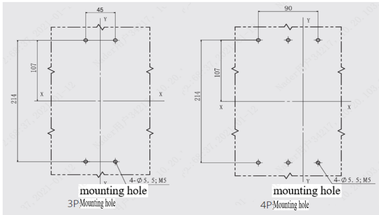
Fig.9 NDM5-250L/M/H 2P 3P 4P Installation dimension drawing of front board wiring products
