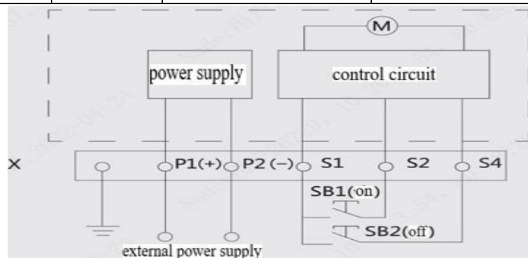
Fig.23 Electric operation wiring diagram
