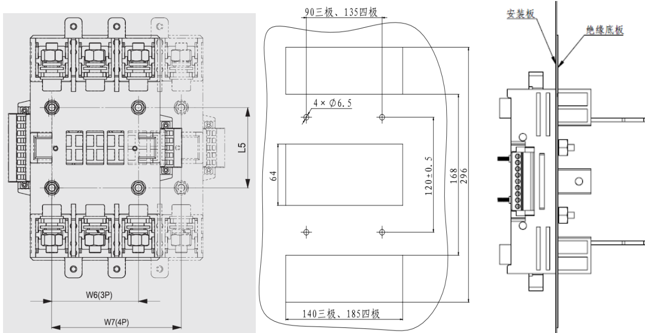
Fig.16 Mounting hole dimensions of plug-in connections
