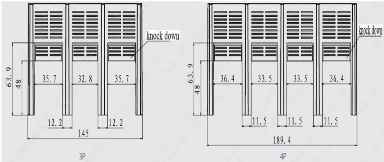
Fig.10 Size of terminal cover
