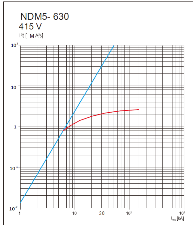
Fig.7 Permissive characteristic curve chart
