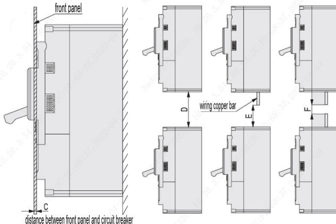
Fig.25 Insulation distance mounted in the metal cabinet
