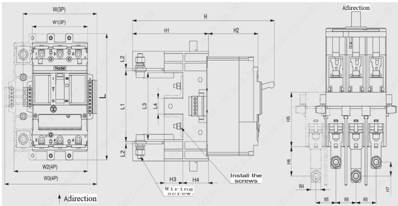
Fig.15 3P、4P Mounting hole dimensions of plug-in connections
