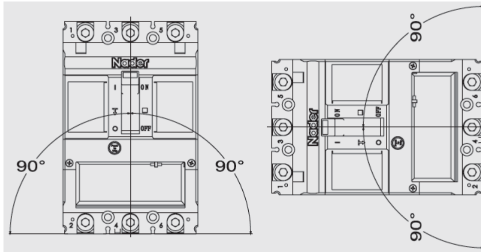
Vertical Installation
