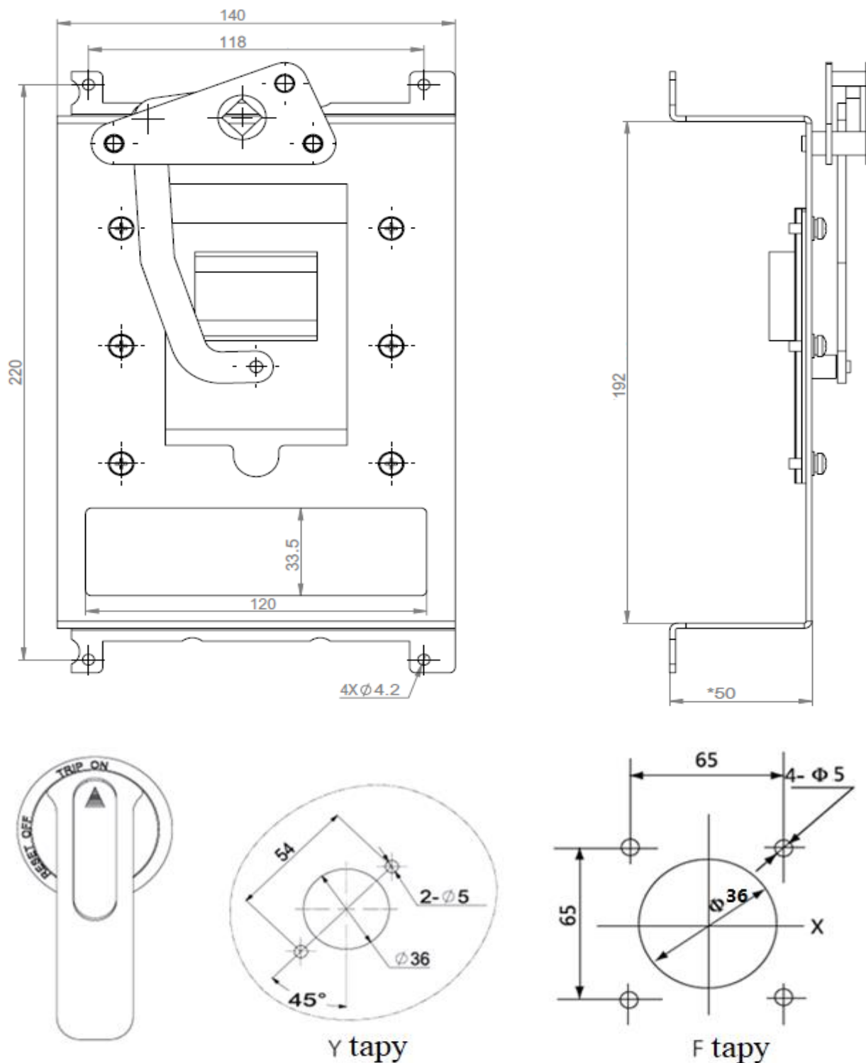
Fig.11 Installation opening diagram of rotary handle
