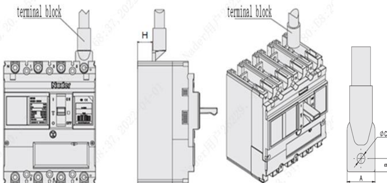
Fig.12 Connection diagram of copper bar in front of board or copper cable with wiring terminal
