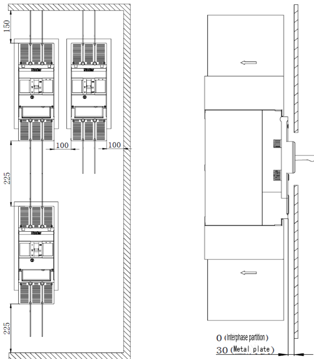
Distance requirement of installation in cabinet
