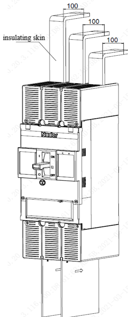
Fig.13 Size of insulated cover
