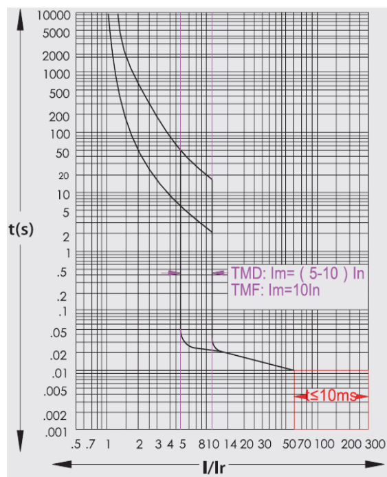
Fig.3 NDM5-630V
