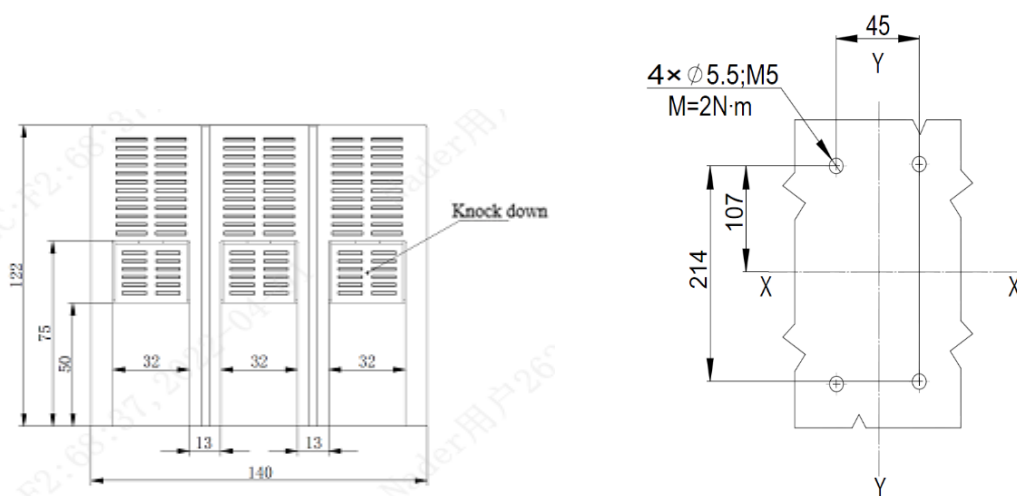
Installation hole size
