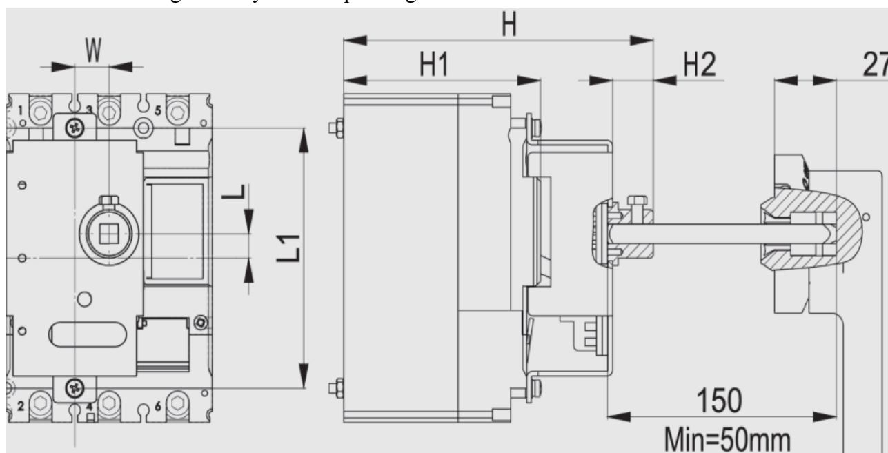
Fig. 10 Installation drawing of rotary handle operating mechanism
