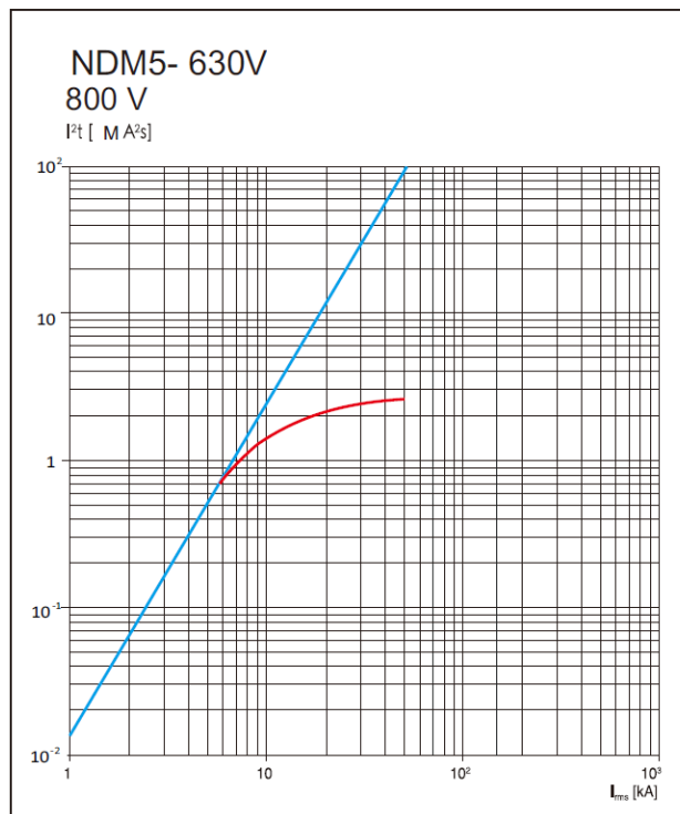
Fig.7 NDM5-630V Permissive characteristic curve chart
