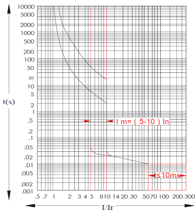
Fig.2 NDM5-400V
