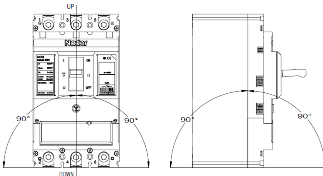
Vertical installation
