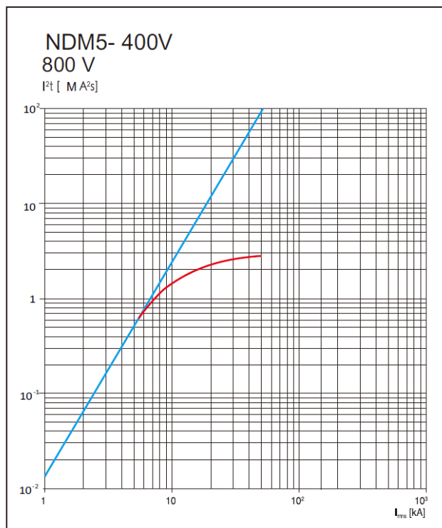
Fig.5 NDM5-400V Permissive characteristic curve chart
