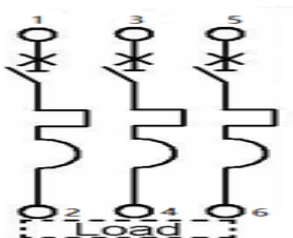
Fig.15 Main circuit wiring mode of AC products
