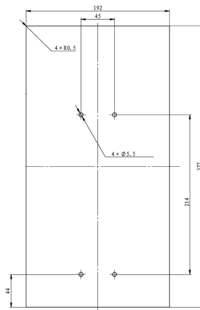
Insulating Plate Dimension
